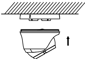
Figure 2-7 Secure the Camera with Mounting Base
