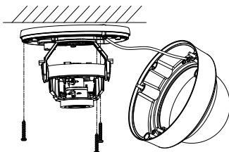
Figure 2-10 Secure the Mounting Base
