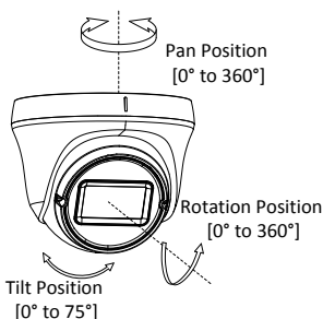
Figure 2-8 3-axis Adjustment
