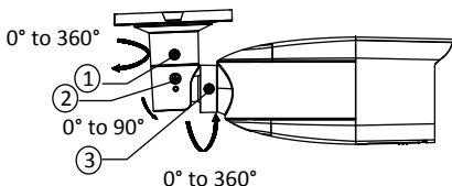
Figure 2-3 3-axis Adjustment
