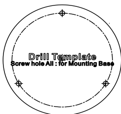
Figure 2-5 Drill Template
