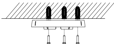
Figure 2-6 Attach the Mounting Base to the Ceiling
