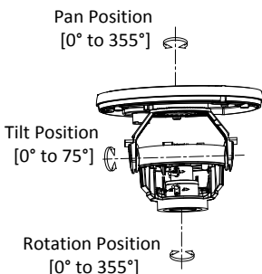
Figure 2-11 3-Axis Adjustment
