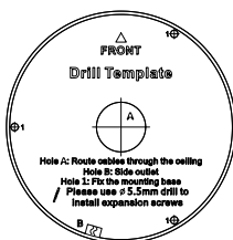
Figure 2-9 The Drill Template
