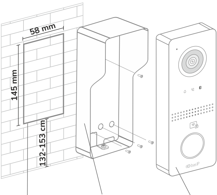
Mounting area
