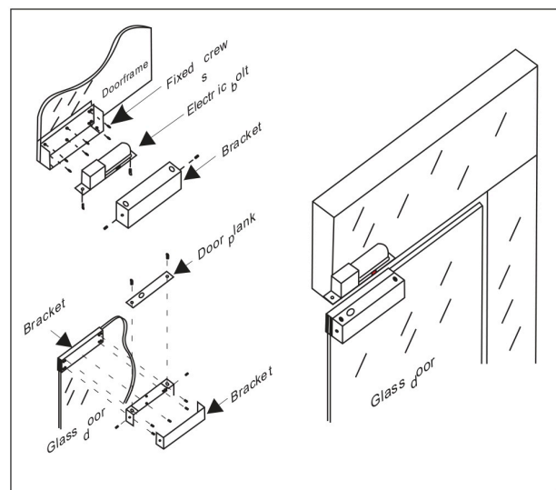
Bracket Installation Diagram
